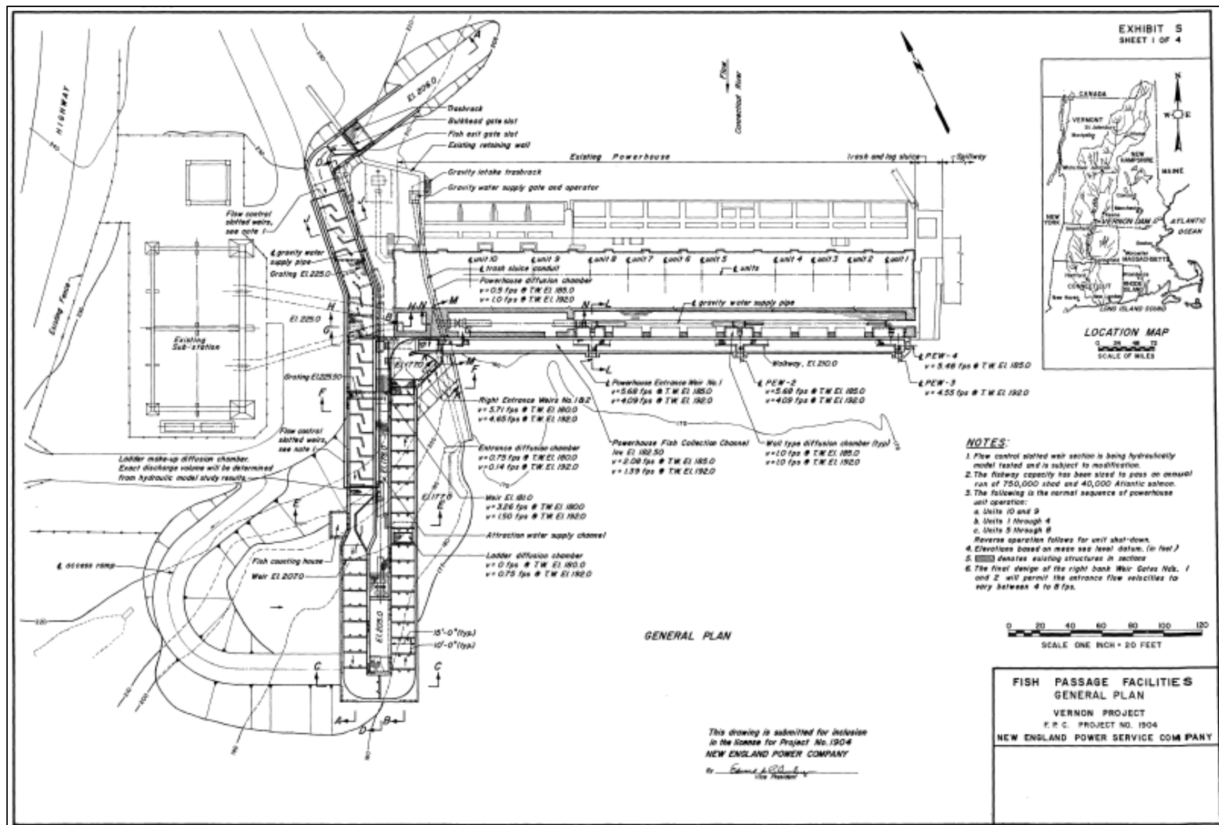
Figure 2.3-7 Fish ladder layout.
